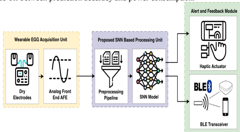
Figure 1. System Architecture of the Wearable Seizure Prediction System
