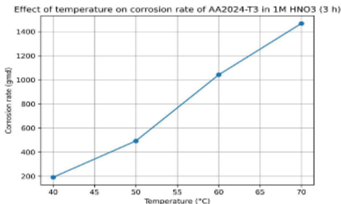
Figure 5. Effect of temperature on the corrosion rate of AA2024-T3 aluminum alloy in 1 M HNO 3 for 3 h.
