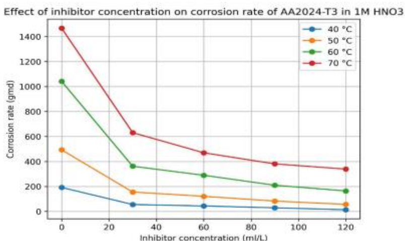
Figure 6. The concentration of inhibitors impacts the corrosion rate of AA2024-T3 aluminium alloys in 1 M HNO 3 in 3 h at different temperatures.
