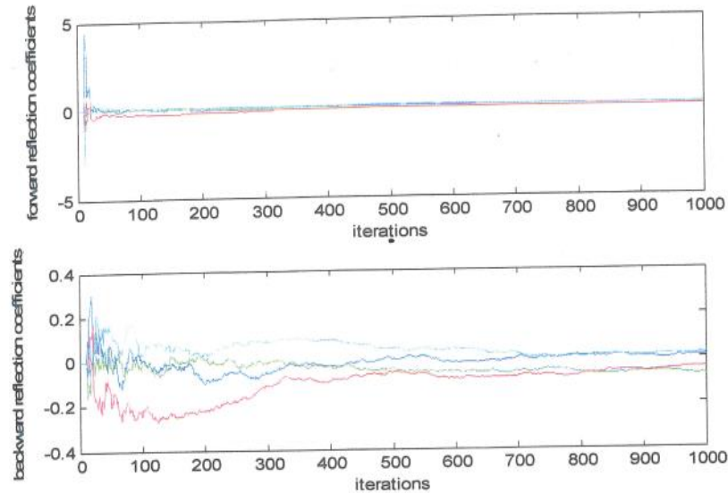
Fig.4 The ensemble average forward and backward reflection coefficients for various channel
