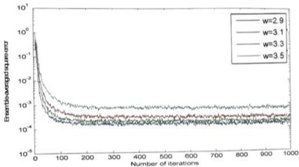
Fig.3 Learning curves of RLSL algorithm for various channels
