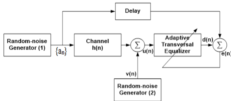
Fig.1 Block diagram of an equalizer
