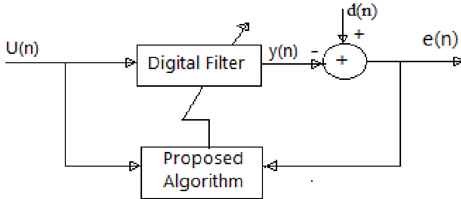
Fig. 2 Block diagram of an Adaptive Equalizer
