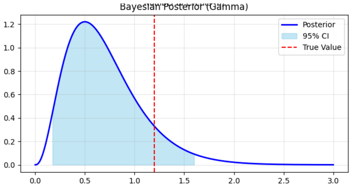
Figure 4: Bayesian Posterior Distribution (Gamma) for a Specific Event Count ( n=3 ) with 95% Credible Interval
