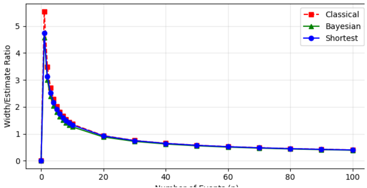
Figure 2: Confidence Interval Width-to-Point Estimate Ratio for Classical, Bayesian, and Shortest Methods
