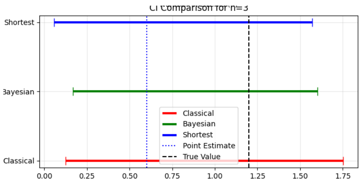
Figure 3: Confidence Interval Comparison for a Specific Event Count (n=3) Using Classical, Bayesian, and Shortest Methods
